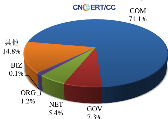
Domain Categories of the Defaced Websites in Mainland China (Dec 24-Dec 30)
